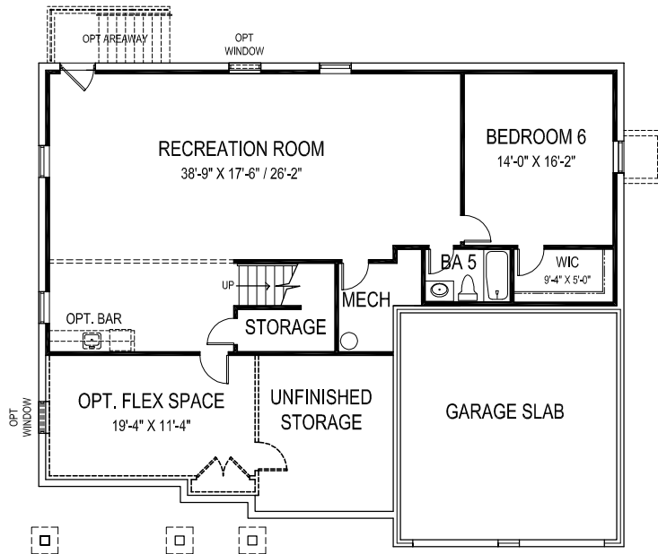
BASEMENT PLAN
